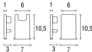
601T005 Tappi (opzionale) Terminals (optional) Verschlüsse (optional) 601T005C Tappi chiusi (opzionale) Closed terminals (optional) Verschlüsse (optional)
