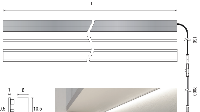
601T005 Tappi (opzionale) Terminals (optional) Verschlüsse (optional) 601T005C Tappi chiusi (opzionale) Closed terminals (optional) Verschlüsse (optional)
